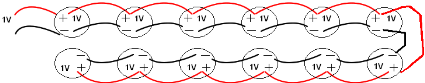
Connecting in Parallel (same voltage, increases capacity [ah])
