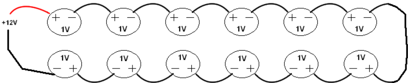
Connecting in Series (increases voltage, same capacity [ah])
